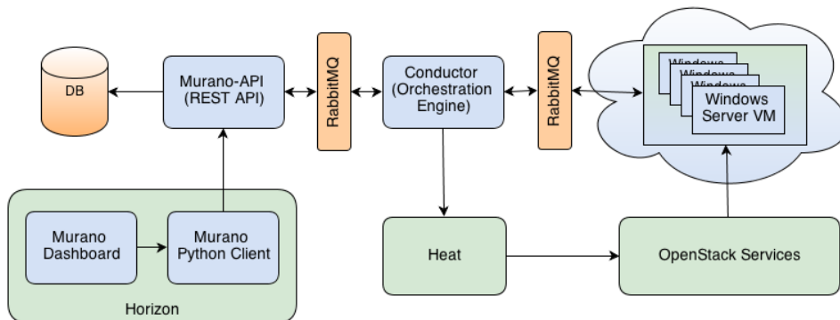
Figure 3.1. Architecture
